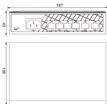
Dimension (mm)
